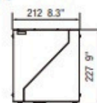
Data Processing Unit WR2120-DPU 2.2 kg 4.5 lb
